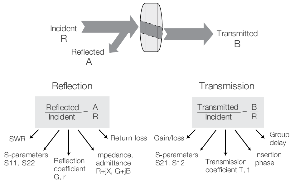
Figure 10. Common terms for high-frequency device characterization
