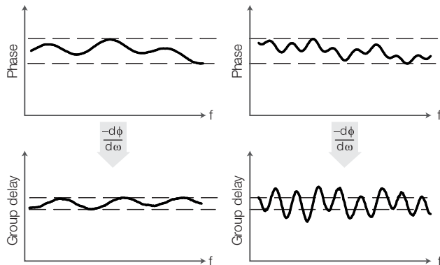
Figure 15. Same peak-to-peak phase ripple can result in different group delay
