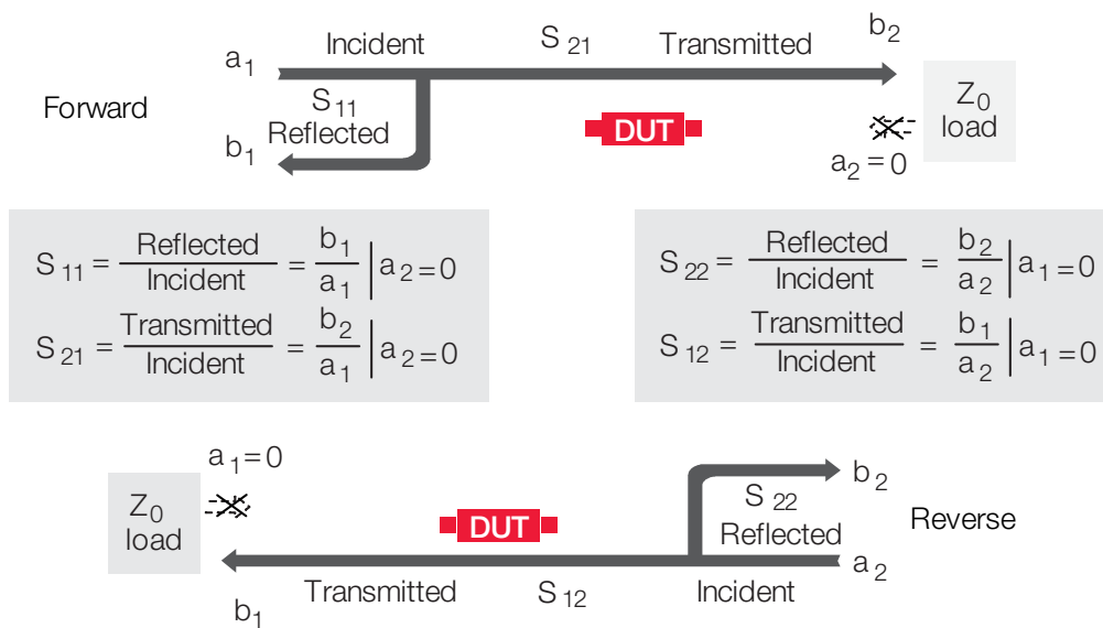
Figure 17. Measuring S-parameters
