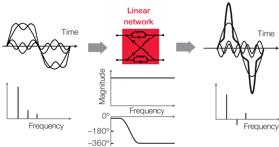
Figure 3. Phase variation with frequency
