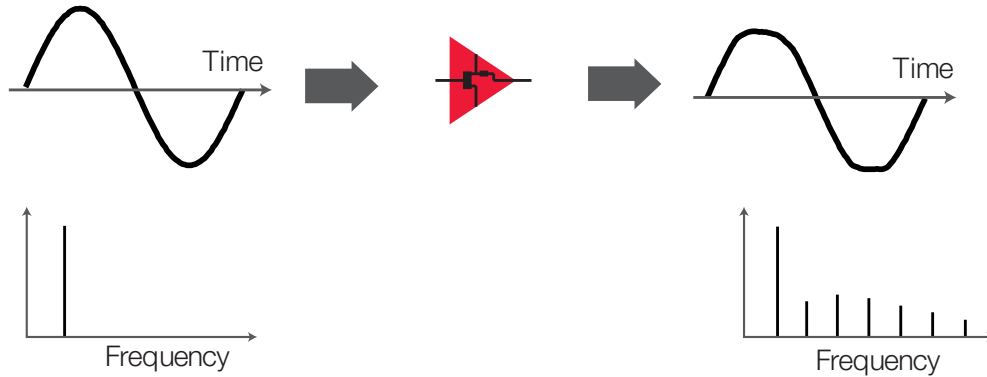
Figure 4. Nonlinear induced distortion
