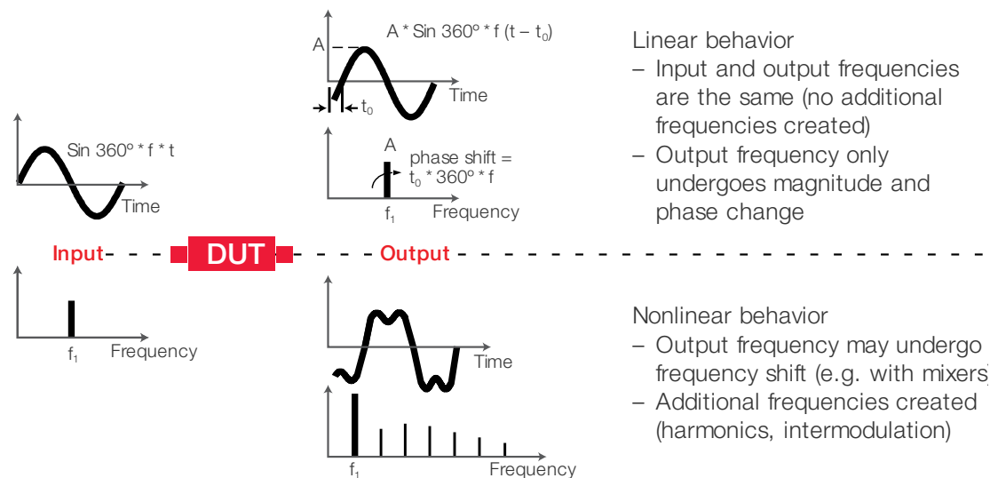
Figure 1. Linear versus nonlinear behavior
